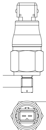
Connettore tipo AMP Junior power timer Connector type AMP Junior power timer
