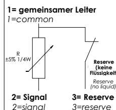
SCHALTPLAN ELECTRICAL SHEET
