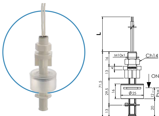
P003AC-1xx / AC-5xx
