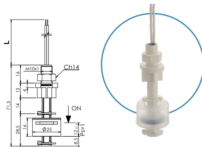
P003AC-2xx / AC-6xx
